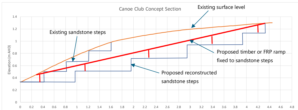
Section view of proposed upgrade, widened sandstone steps with FRP panels. Existing surface level derived from Spatial Services, Department Finance, Services and Innovation, 1 m Digital Elevation Model derived from LIDAR, April 2013.
